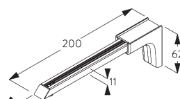
SG 11156 Smart fix universale 200 mm
