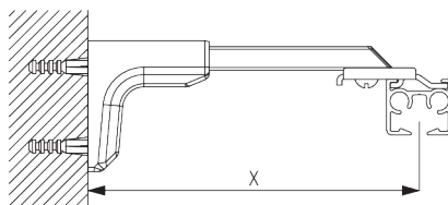
Smart Fix universale SG 11154 - SG 11156 e supporto SG 3832:
