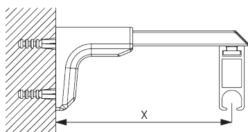
Smart Fix universale SG 11154 - SG 11156 e SG 6141: Necessaria vite SG 11131 (M4x6).
