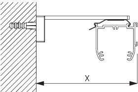
Smart Fix squadrato SG 11210 - SG 11215 e supporto SG 2616: Necessaria vite SG 10395 (M4x6).
