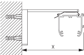
Smart Fix SG 11200 - SG 11205 e supporto SG 2616: Necessaria vite SG 10395 (M4x6).
