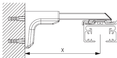
Smart Fix universale SG 11154 - SG 11156 e supporto girevole SG 3044: Necessaria vite SG 10492 (M4x8).
