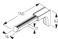
SG 11155 Smart fix universale 150 mm
