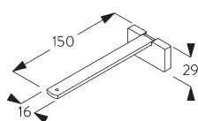
SG 11214 Smart Fix squadrato 150 mm
